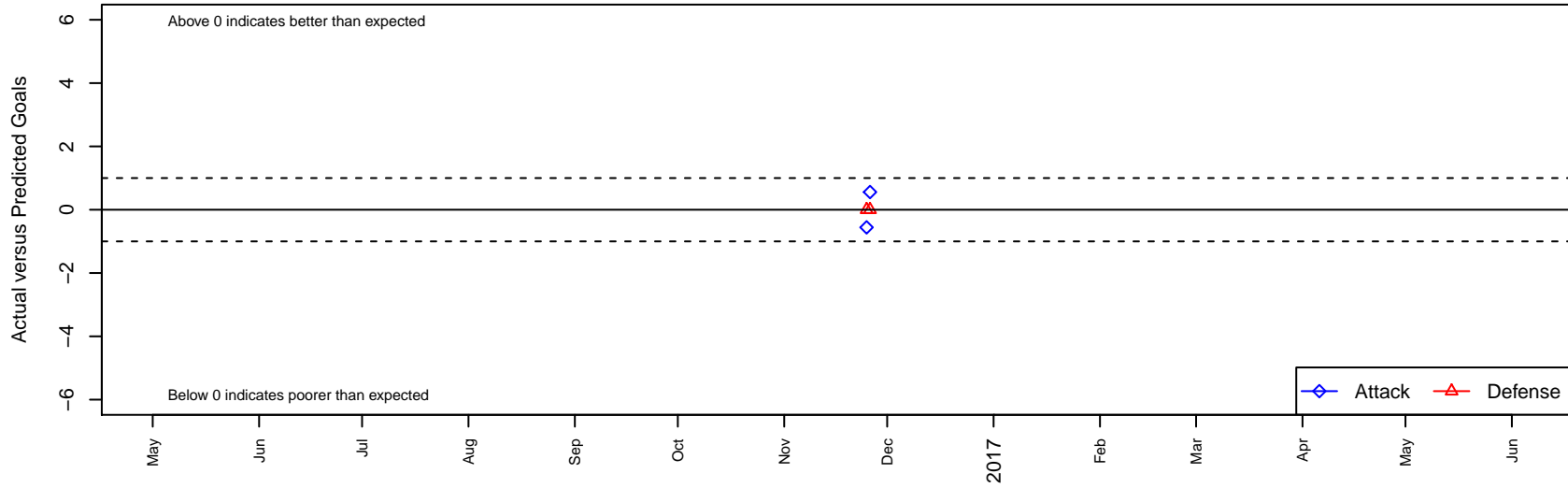
Pride SC Predators B99 Dots are actual minus expected GF (blue circles) and GA (red triangles). Blue line is smoothed change in attack strength. Red is smoothed change in defense strength.
